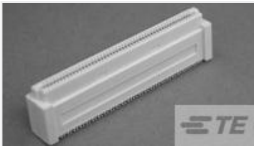
TE 产品编号5084616-5 0.8FH,R13H.5,120,08/Sn,TR,SC
