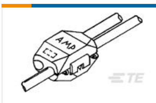
TE 产品编号53440-2 ELECTRO-TAP, 20-18 AWG RUN&TAP
