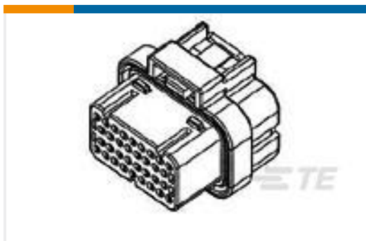
TE 产品编号3-1437290-8 26POS,SUPERSEAL,REC HSG ASSY, SLD,COD 2
