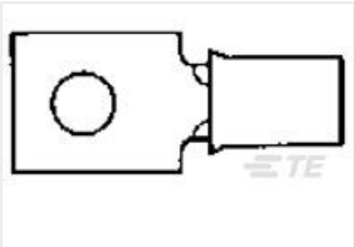
TE 产品编号61359-1 RING GR ANTI ROTATIONAL 18-14 AWG PTPST
