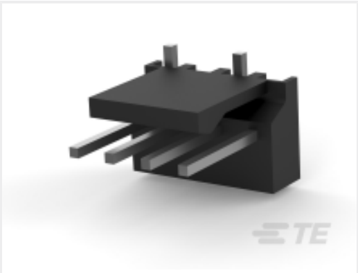
TE 产品编号1744382-8 08P MTA100 HDR ASSY,SM,SN, LF
