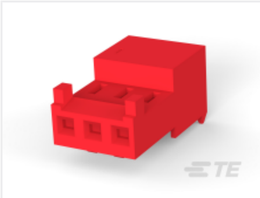
TE 产品编号CAT-104MTA-NTPMR Nylon Tin Plated Receptacle: 2.54 mm, with Mating Alignment, MTA 100
