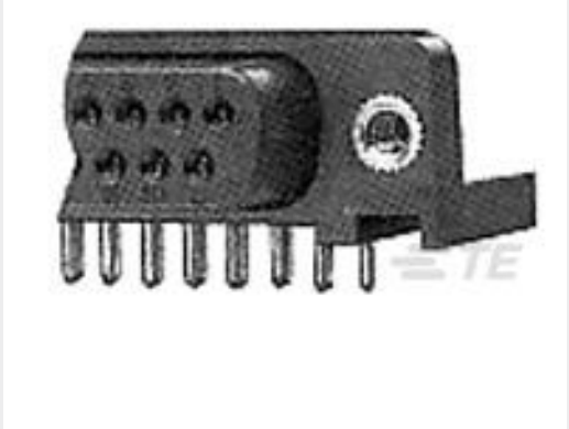
TE 产品编号5748901-1 AMP III RCPT 25P RA 318 THD IN
