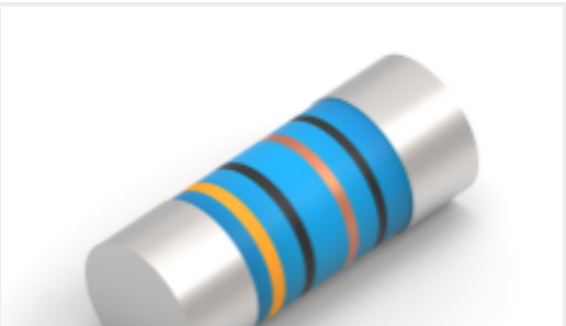
TE 产品编号5-2176315-2 MELF SMA_A 1K5 1% 50PPM 0204 0.4 W
