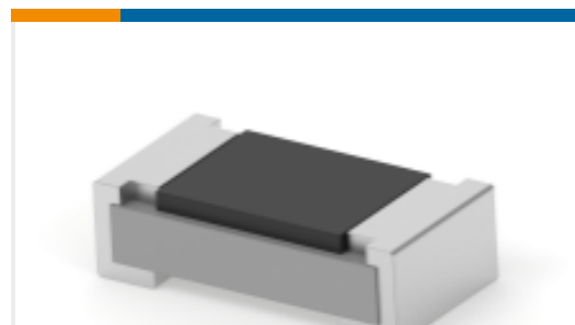
TE 产品编号2176237-8 CPF A 0603 33R 0.1% 25PPM 5K RL
