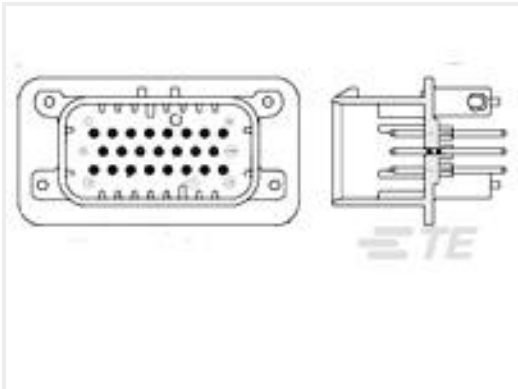
TE 产品编号776231-5 35POS,PIN DIA 1.3,HDR ASSY, 180DEG,COD 5
