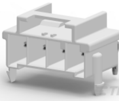
TE 产品编号1-1969694-4 PTL 1X4 PCB HEADER R/A HITEMP KEY A LGR
