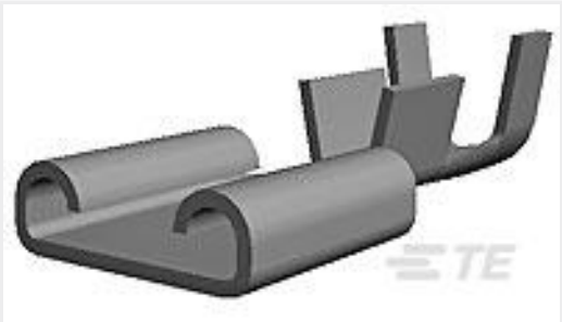
TE 产品编号160916-3 250 FASTON,REC.,17-14 AWG,PB
