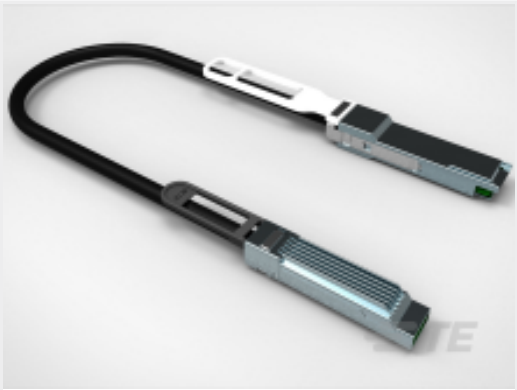
TE 产品编号 2821782-2 MICROQSFP TO QSFP28, 1M 28AWG
