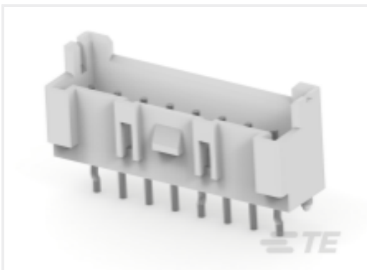
TE 产品编号2404280-8 EP 2.5 HDR, GLOW WIRE, 8P
