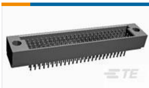
TE 产品编号532448-5 HDI PIN ASSY 4 ROW 160 POS
