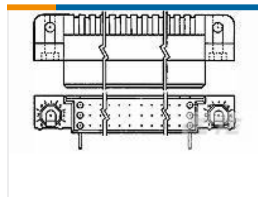
TE 产品编号533268-1 HDI RECP ASSY 3 ROW 75 POS
