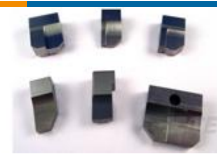
TE 产品编号7-1633139-4 ANVIL, COMBINATION PREMIUM
