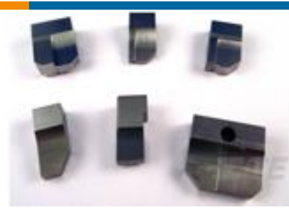
TE 产品编号3-1333205-9 ANVIL, COMBINATION .090
