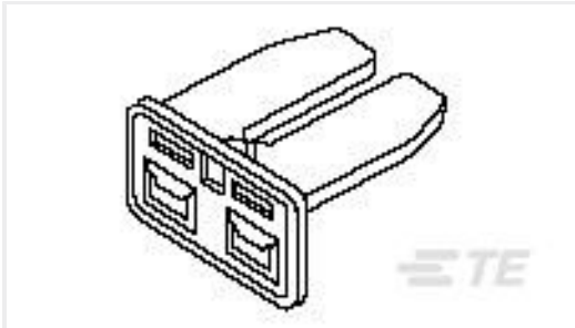
TE 产品编号174353-7 070 ECONOSEAL MARK-2 PLATE 2P
