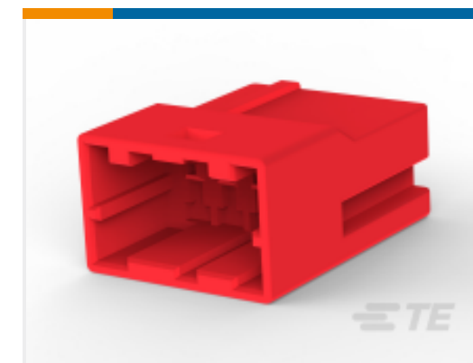
TE 产品编号 1-1903393-2 GIC 2.5 W CAP HSG 4P RED
