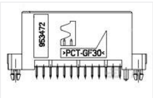
TE 产品编号953472-1 26pos MQS .63 header 180deg THR
