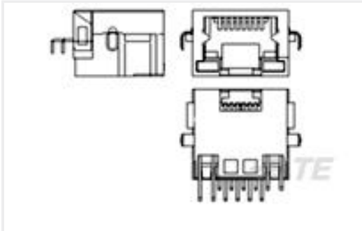
TE 产品编号2041411-1 RJ45 w/ LED, Tab Up, Offset, DIP, H=9.45
