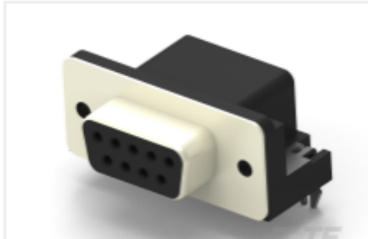
TE 产品编号2301844-1 AMPL REC HD20, R/A, 9P, B/L,4-40 INS
