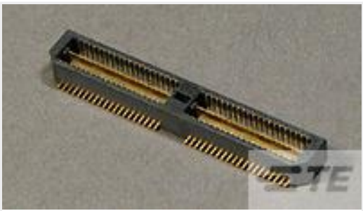
TE 产品编号1-1658013-2 MSB0.80PL5ASY56DP,-,10,VCTY
