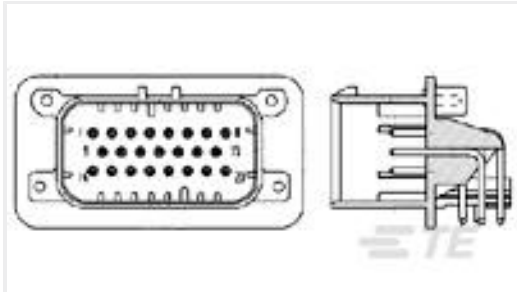
TE 产品编号1-776087-2 23POS,PIN DIA 1.3,HDR ASSY,90DEG, COD 2
