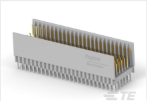
TE 产品编号3-100669-0 2MM HM TYPE B PIN ASSEMBLY
