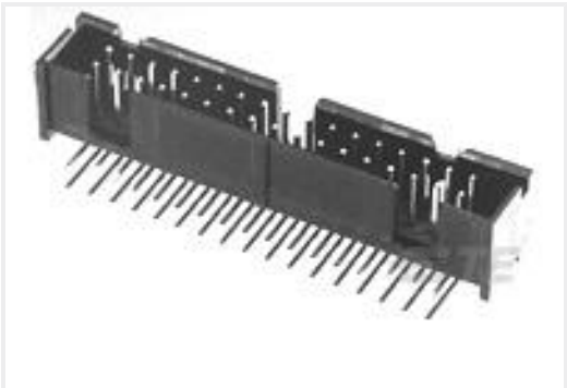
TE 产品编号5103310-6 A/L LOW PRO HDR 26P RA BLACK
