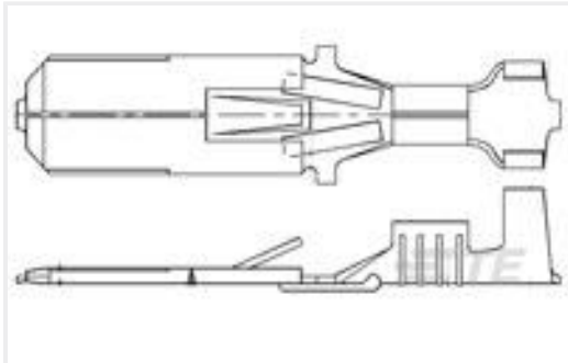
TE 产品编号42241-2 FF 250 TAB 18-14 AWG .032 TPBR
