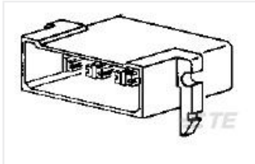
TE 产品编号163008 FF 250 TAB HSG 8P NYLON CLEAR
