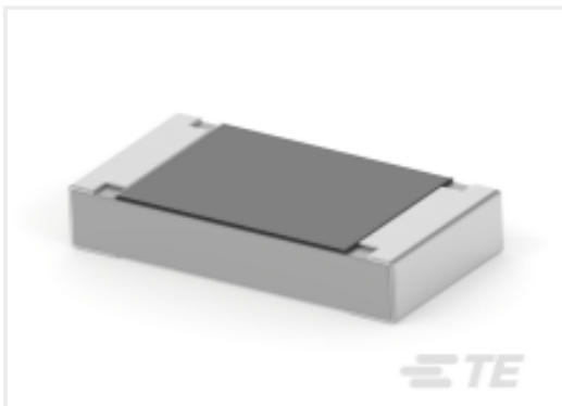
TE 产品编号2-2176344-5 CRGCQ 1206 10K 5%
