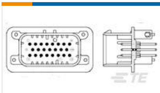
TE 产品编号1-776228-1 23POS,PIN DIA 1.3,HDR ASSY, 180DEG,COD 1
