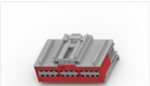
TE 产品编号1-1452839-5 24 POS FEMALE HSG ASSY
