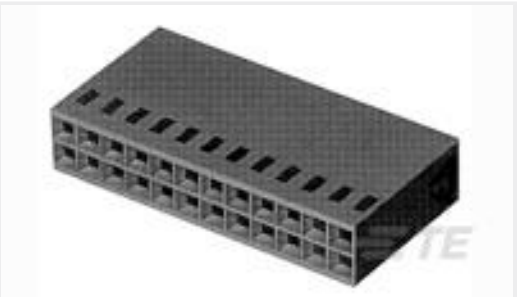
TE 产品编号2-87456-3 28 MODIV HSG COMP DR .100CL
