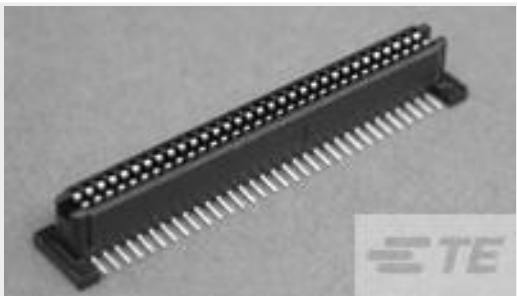
TE 产品编号120528-1 1FHR,64,30A/P,N,C,S08,09,10
