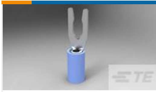
TE 产品编号52420-1 TERMINAL,PIDG SPR SPD 16-14 6
