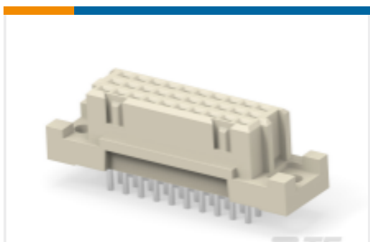
TE 产品编号254320-E STVC/3 30 F ABC VV 7-00 TL 4,0 * 247 E0
