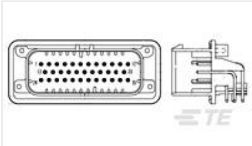
TE 产品编号776163-5 35POS,PIN DIA 1.3,HDR ASSY,90DEG, COD 5
