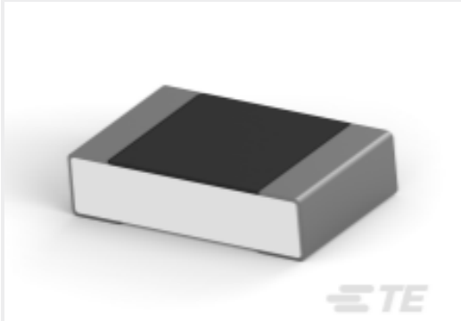
TE 产品编号2-2176382-4 RQ 0805 232K 0.1% 10PPM 5K RL
