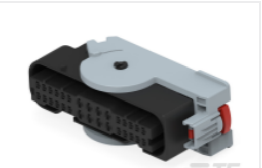
TE 产品编号5-2109446-2 MCP 1.5/2.8 SLD 30P PLUG ASSY
