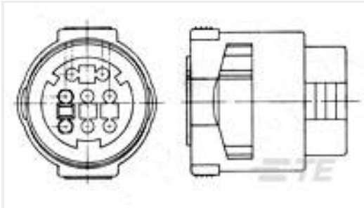
TE 产品编号172191-2 ECONOSEAL-J CONN PLUG 8P BLACK
