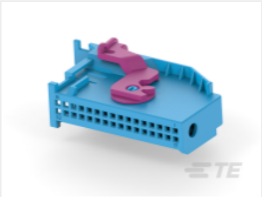
TE 产品编号2050723-2 COVER FOR MQS HSG 2x16 POS ASSY
