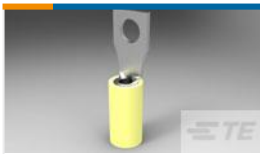
TE 产品编号2-327960-2 TERMINAL,PIDG RECT 12-10 6
