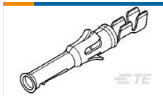
TE 产品编号66592-4 TYPE VI SKT,MULTI-MATE,L.P.
