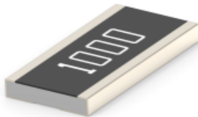
TE 产品编号3-2176566-2 3430 A3 1% 18R 200ppm 1k RL
