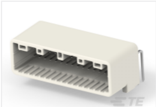
TE 产品编号2326784-3 32POS,TAB0.64X0.64,HDR ASSY,90DEG,SLDR
