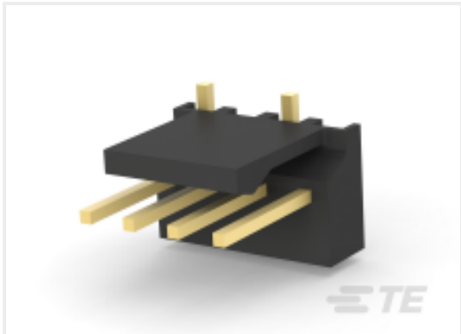
TE 产品编号3-1744163-4 04P MTA100 HDR ASSY SM 30AU LF
