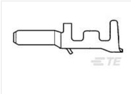
TE 产品编号917571-1 1.5 BTW POST CONTACT
