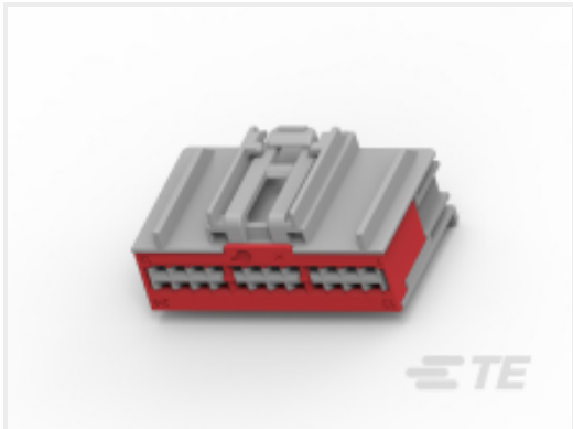
TE 产品编号1-1452839-5 24 POS FEMALE HSG ASSY
