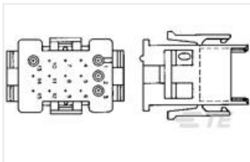
TE 产品编号1-640515-0 24P MR II CAP HSG V0
