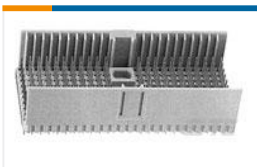
TE 产品编号5646346-1 2MM HM,ASY,T-D,HDR,8R,176P,AP
