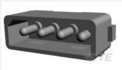
TE 产品编号350424-1 04P CMNL HDR ASSY PC NATL
