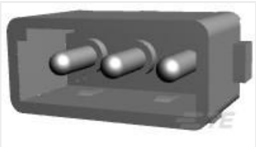
TE 产品编号350423-1 03P CMNL HDR ASSY PC NATL
