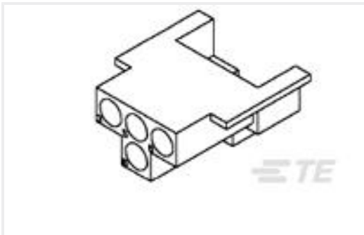
TE 产品编号880125 9 CIR CAP 140DIA PANEL MT NAT
