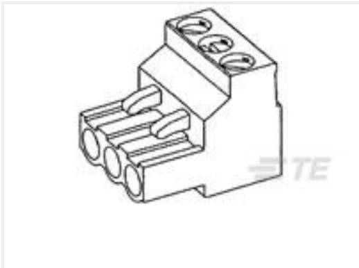
TE 产品编号796640-2 2 POS 5.0 MM R/A PLUG,TRM BLK
