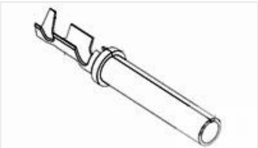
TE 产品编号776492-1 SOC, SF, SIZE 16, 14-18 AWG, AU/SN
